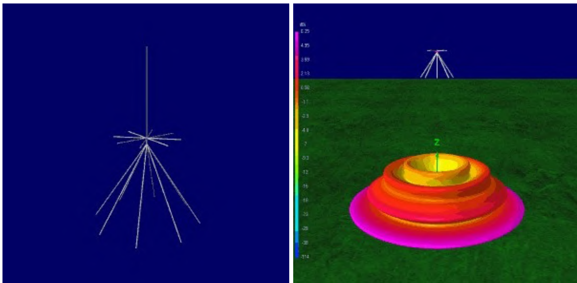
Left: Image of a typical discone with whip, Right: 3D Radiation Pattern at 144
