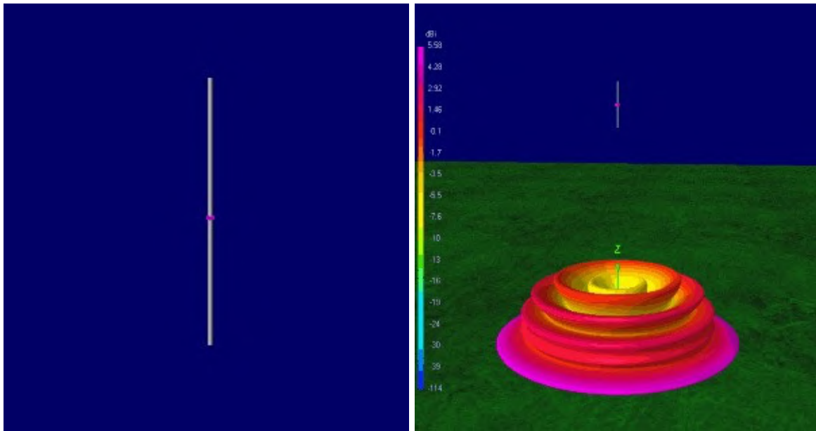
Left: Image of a typical dipole, Right: 3D Radiation Pattern at 144 MHz and 5m high
