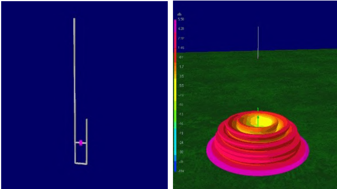
Left: Image of a typical j-pole, Right: 3D Radiation Pattern at 144 MHz and 5m
