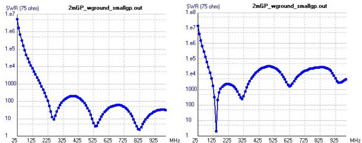
Left: Whip with ground plane of 1cm. Right: Whip with ground plane of 1cm and 2.23 uH loading coil at the base.
